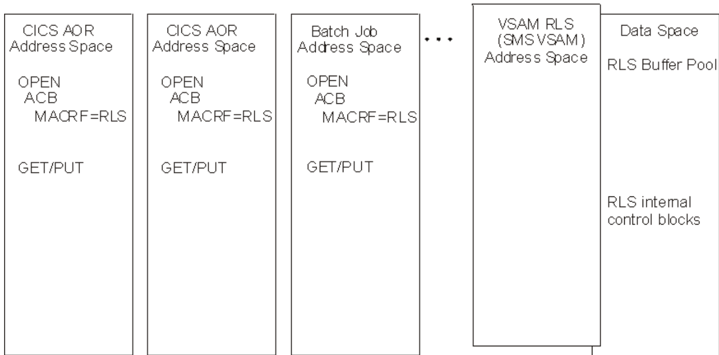
Figure 1: VSAM RLS address and data spaces and requestor address spaces
